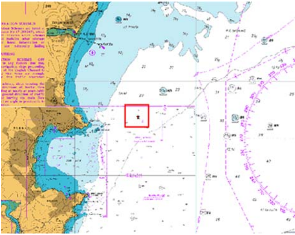
Fig. 1.1 Initial position of the wreck plotted
