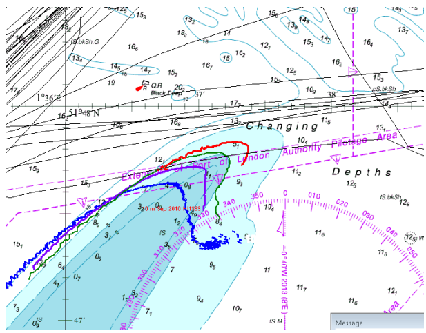
Fig. 2.1 5 metres contours over a 4 year period Fig. 2.2 Original traffic patterns with contours
