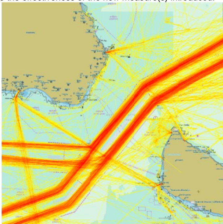
Fig. 5 AIS density plot after the implementation of TSS Bornholmssgat between Denmark and Sweden
