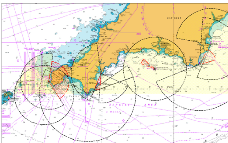
Fig. 3.1 An example of adjacent lighthouses showing range and sector details
