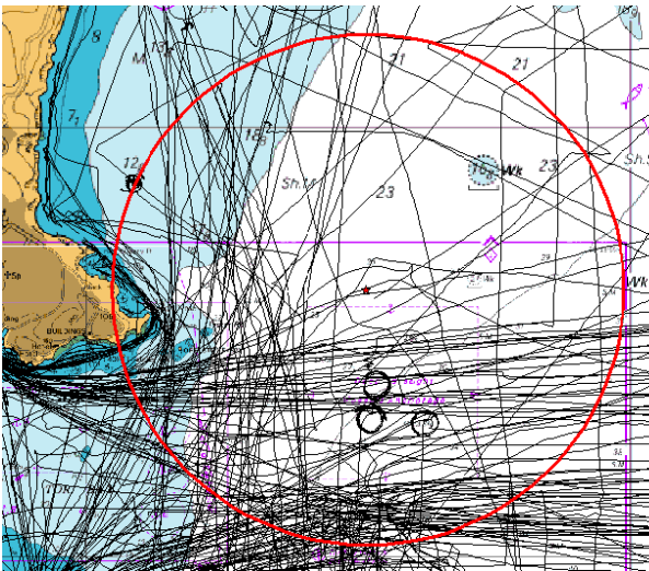
Fig. 1.3 Vessels passing within 3nm of the wreck
