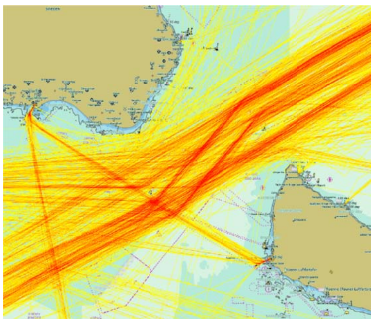
Fig. 4 AIS density plot before the implementation of Traffic Separation Scheme (TSS) Bornholmsgat between Denmark and Sweden
